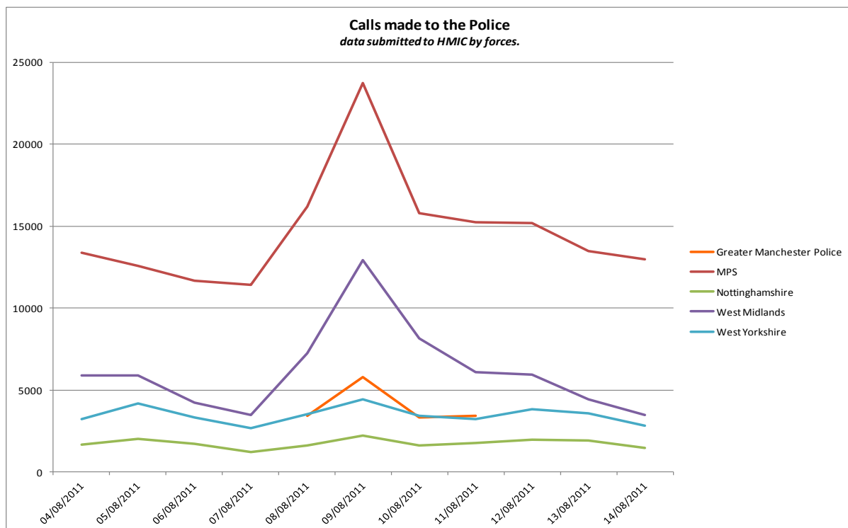
Figure 5 Calls made to the police over the riot period (Greater Manchester, London, Nottinghamshire, West Midlands and West Yorkshire)
